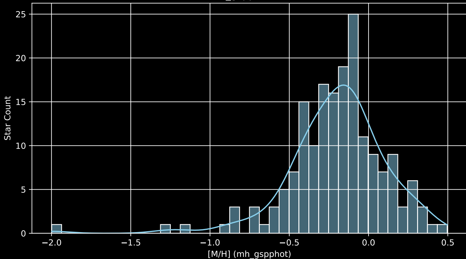
APOGEE DR17 Field: [055+33_MGA [M/H] (mh_gspphot) (n= 178)
