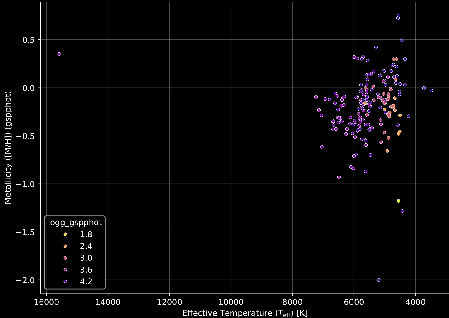
APOGEE DR17 Field: [055+33_MGA] Stellar Population Parameters (n= 180)
