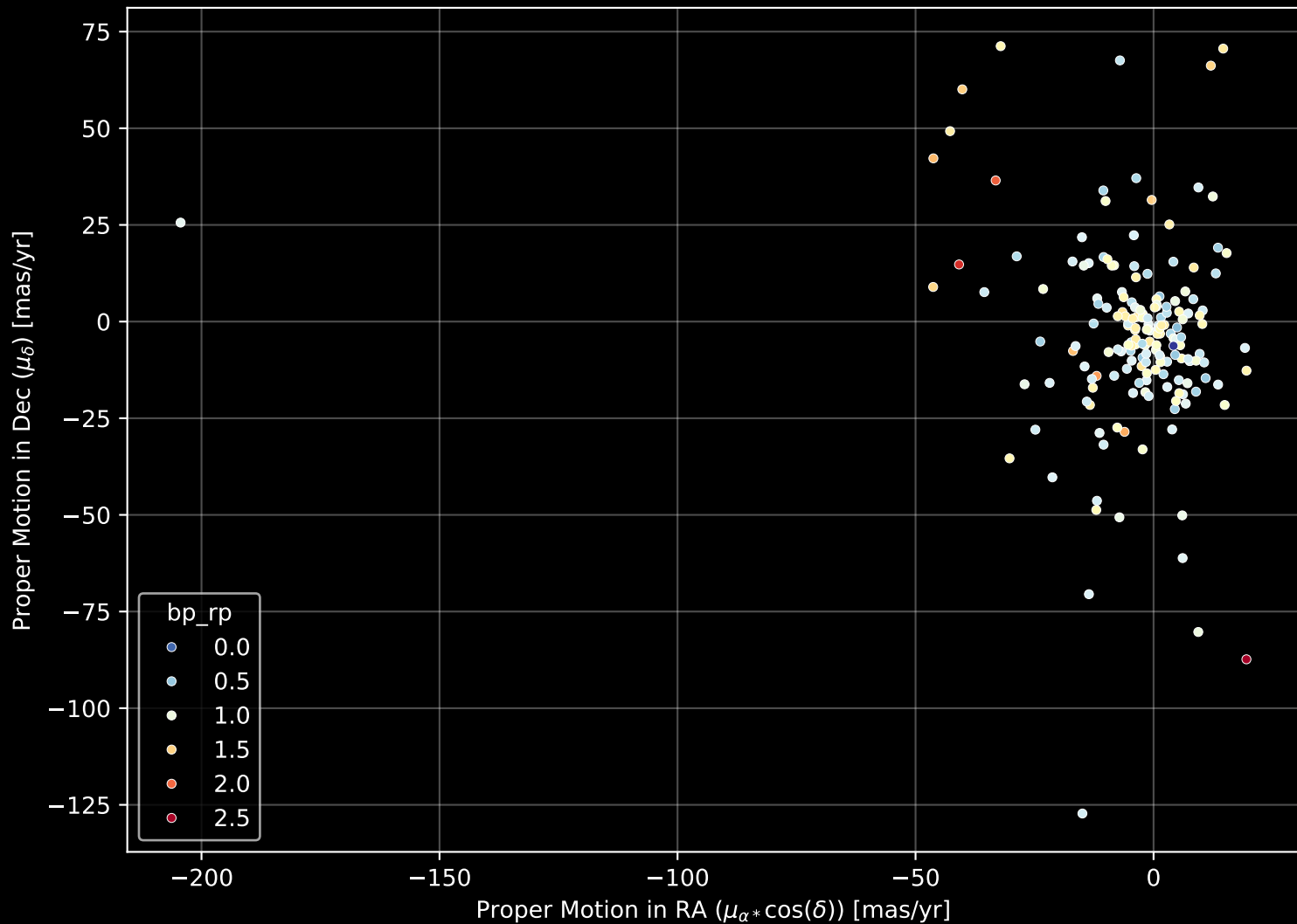
APOGEE DR17 Field: [055+33_MGA] Proper Motion Diagram (n= 180)
