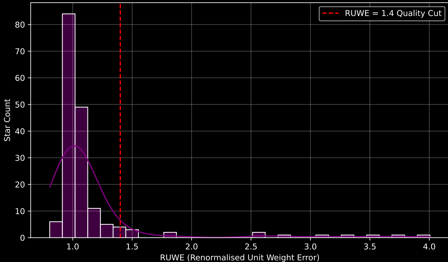
GAPOGEE DR17 Field [055+33_MGA] RUWE Distribution (n= 172)
