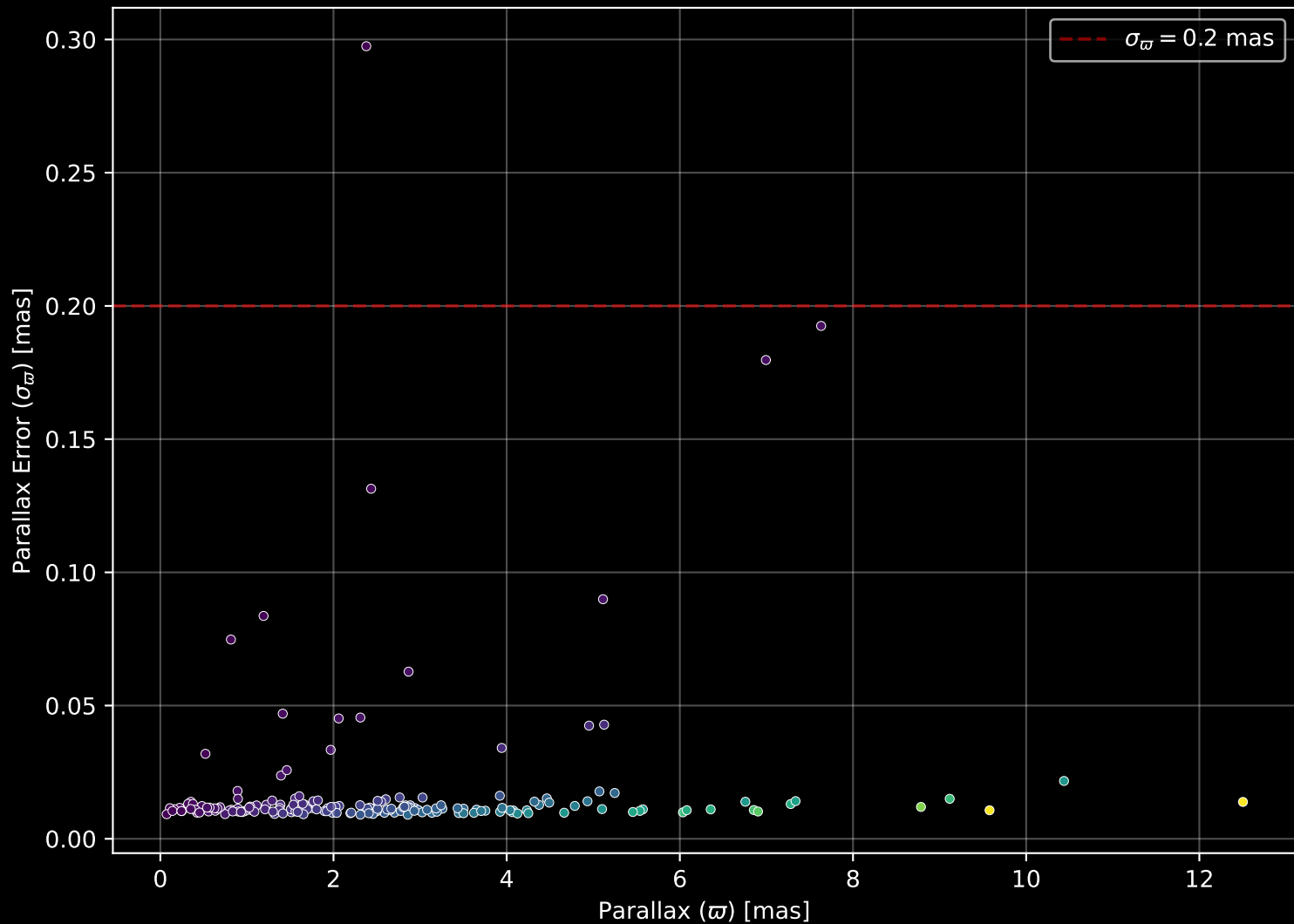
APOGEE DR17 Field: [055+33_MGA] Parallax Quality (n= 180)
