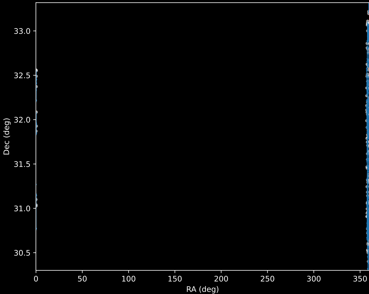
APOGEE DR17 Cluster 0 Proper Motion Vectors (n=110)
